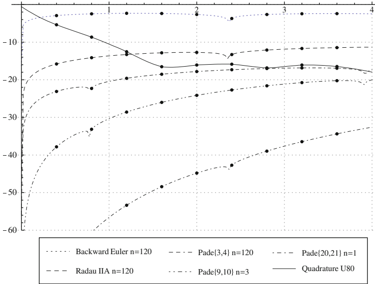
Figure 1. Logarithmic error \log_{10}(E(n, t, u)) for different schemes provided by Padé approximants and the quadrature method U80 (see Table 1 of [39]) for the approximation of the solution u of (16) for t \in [0, 4]
